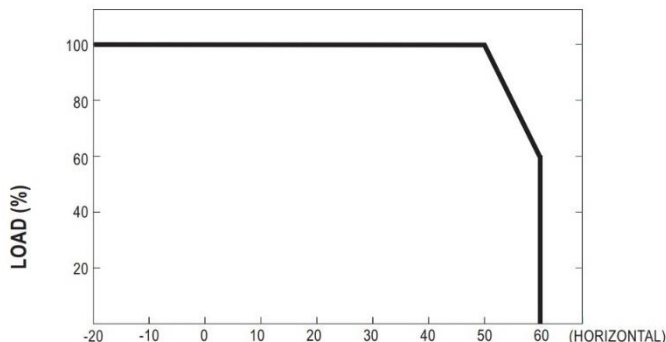
■ Derating Curve
